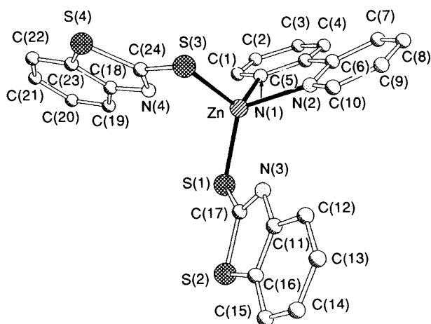
Fig. 2 Structure of [\text{Zn}(\text{C}_7\text{H}_4\text{NS}_2)_2(\text{bipy})] \mathbf{2} and numbering scheme
