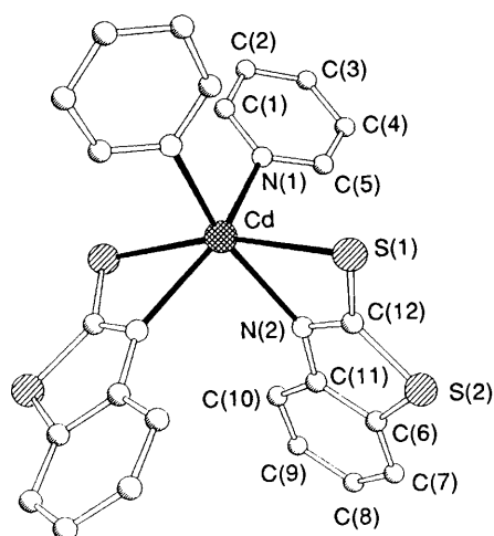
Fig. 3 Structure of [\text{Cd}(\text{C}_7\text{H}_4\text{NS}_2)_2(\text{py})_2] \mathbf{3} and numbering scheme
